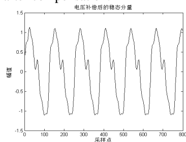
Figure 11. Stable signal component after voltage compensation)
