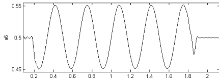
Figure 16. Reconstruction low frequency signal a6
