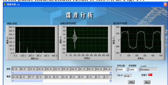
Figure 17. Harmonic analysis front panel
