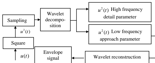
Figure 7. Wavelet transforms measurement
