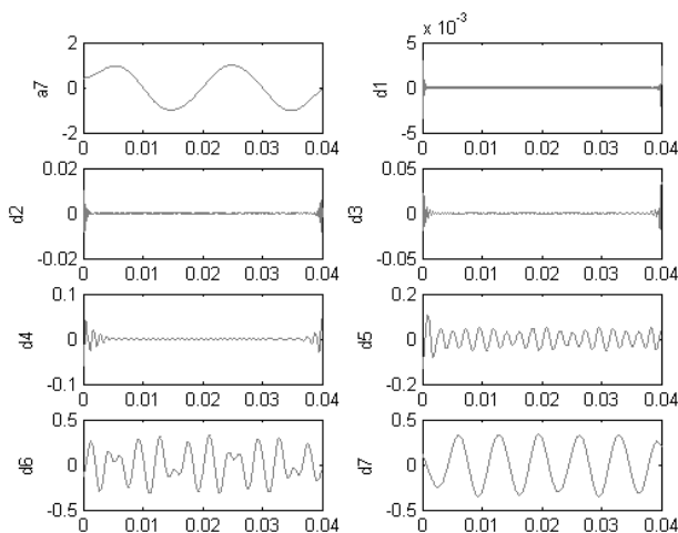
Figure 12. Reconstructed of various wavelet resolution coefficients
