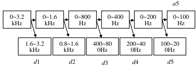
Figure 9. Dividing of signal y frequency band.
