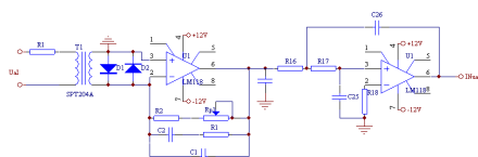
Figure 2. Voltage transformer circuit
