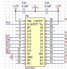
Figure 3. Multi-channel selection switch circuit
