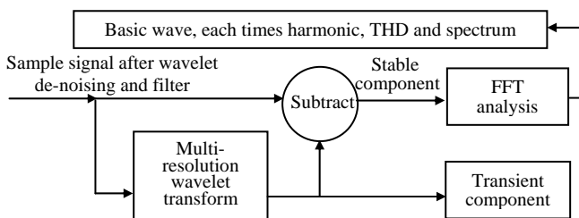
Figure 6. Flow diagram of combining wavelet transform with FFT
