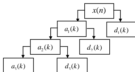
Figure 5. Multi-resolution wavelet decomposition
